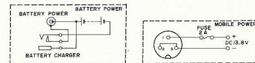
SCHEMATIC DIAGRAM MODEL SELECT TRANSCEIVER AM-FM 160 CHANNEL
