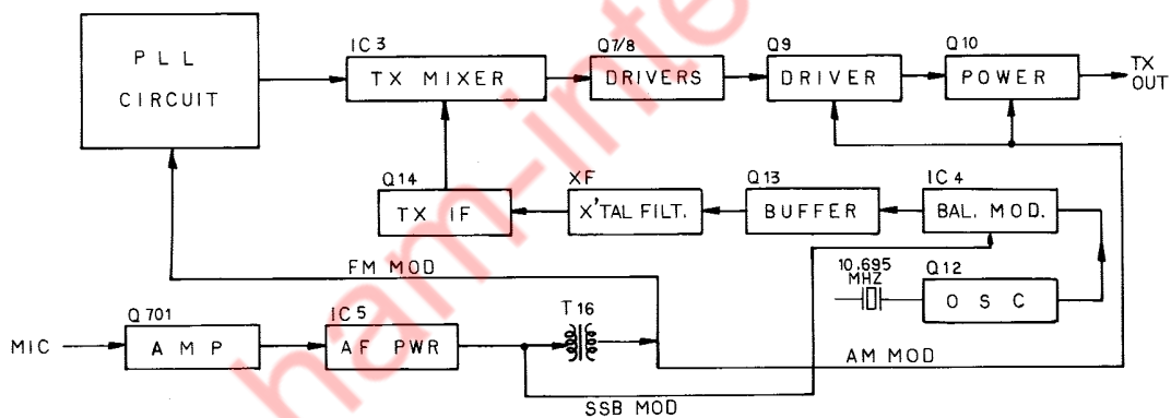
TX Diagram
